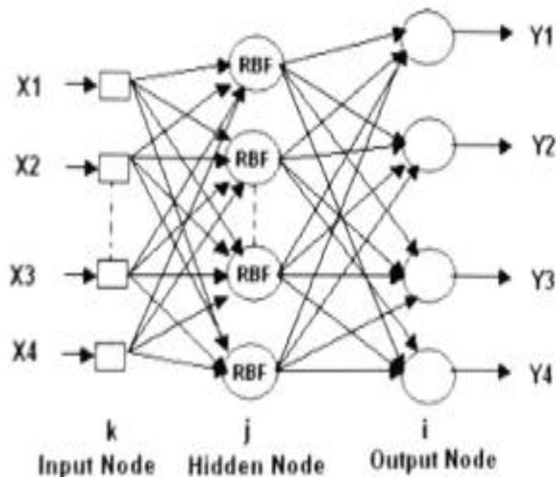
Figure 2 RAN Architecture
