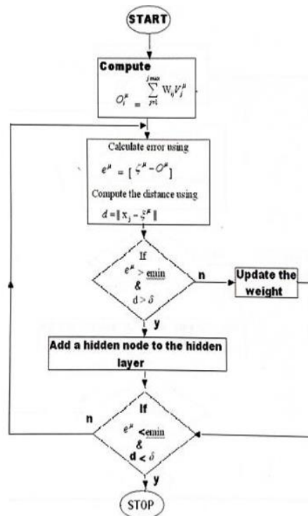
Figure 3 Flow Chart of The RAN Algorithm
