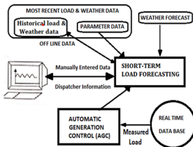
Figure 1 :Input Data for Short Term Load Forecasting
